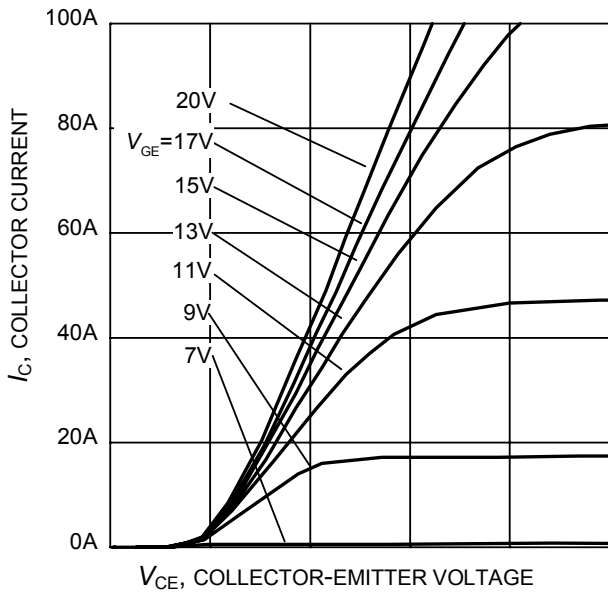
Figure 5. Typical output characteristic ( T_j = 25^\circ\text{C} )
