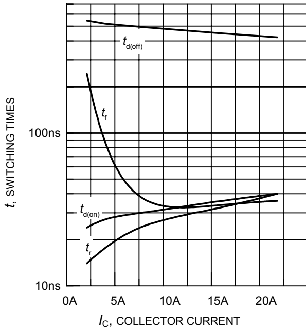
Figure 9. Typical switching times as a function of collector current (inductive load, T_j = 150^{\circ}\text{C} , V_{\text{CE}} = 800\text{V} , V_{\text{GE}} = +15\text{V}/0\text{V} , R_G = 47\Omega , dynamic test circuit in Fig.E )
