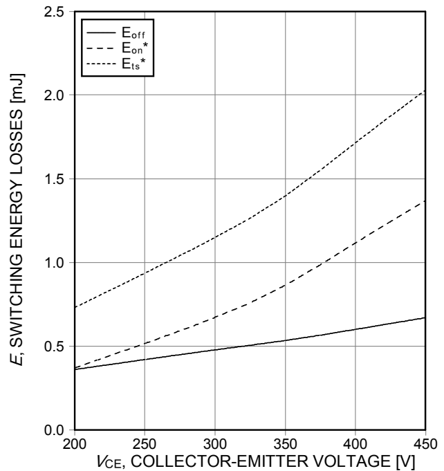
Figure 16. Typical switching energy losses as a function of collector emitter voltage (ind. load, T_j=175^\circ\text{C} , V_{GE}=15/0\text{V} , I_c=30\text{A} , R_G=10,5\Omega , test circuit in Fig. E)
