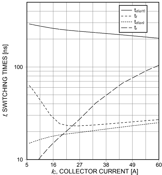
Figure 9. Typical switching times as a function of collector current (ind. load, T_j=175^\circ\text{C} , V_{CE}=400\text{V} , V_{GE}=15/0\text{V} , R_G=10,5\Omega , test circuit in Fig. E)
