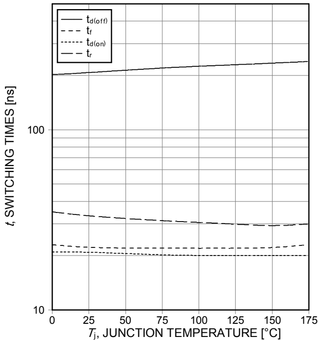
Figure 11. Typical switching times as a function of junction temperature (ind. load, V_{CE}=400\text{V} , V_{GE}=15/0\text{V} , I_C=30\text{A} , R_G=10,5\Omega , test circuit in Fig. E)
