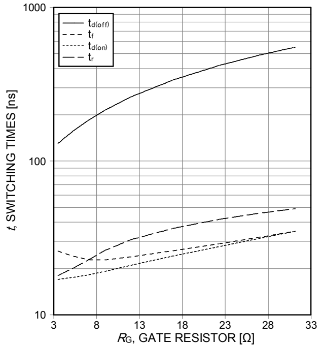
Figure 10. Typical switching times as a function of gate resistor (ind. load, T_j=175^\circ\text{C} , V_{CE}=400\text{V} , V_{GE}=15/0\text{V} , I_C=30\text{A} , test circuit in Fig. E)
