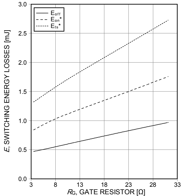
Figure 14. Typical switching energy losses as a function of gate resistor (ind. load, T_j=175^\circ\text{C} , V_{CE}=400\text{V} , V_{GE}=15/0\text{V} , I_c=30\text{A} , test circuit in Fig. E)
