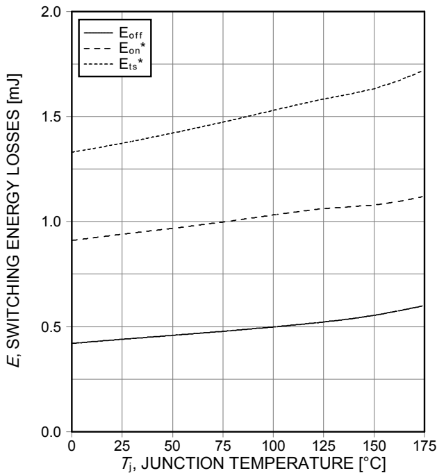
Figure 15. Typical switching energy losses as a function of junction temperature (ind. load, V_{CE}=400\text{V} , V_{GE}=15/0\text{V} , I_c=30\text{A} , R_G=10,5\Omega , test circuit in Fig. E)
