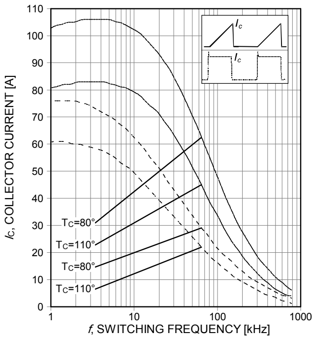
Figure 1. Collector current as a function of switching frequency ( T_j \leq 175^\circ\text{C} , D=0.5 , V_{CE}=600\text{V} , V_{GE}=15/0\text{V} , R_G=10,5\Omega )
