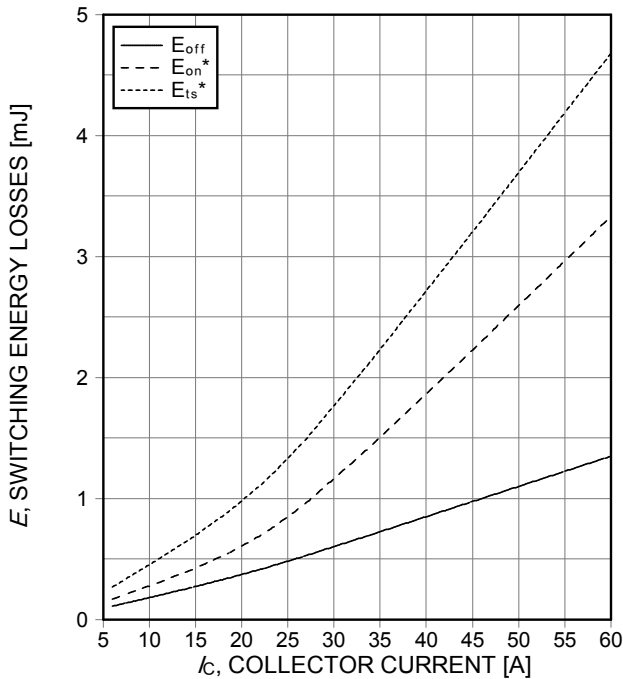
Figure 13. Typical switching energy losses as a function of collector current (ind. load, T_j=175^\circ\text{C} , V_{CE}=400\text{V} , V_{GE}=15/0\text{V} , R_G=10,5\Omega , test circuit in Fig. E)
