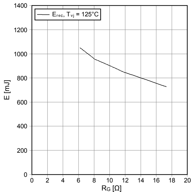
Schaltverluste Diode-Brems-Chopper switching losses Diode-brake-chopper E_{rec} = f(R_G) I_F = 400\text{ A}, V_{CE} = 3600\text{ V}
