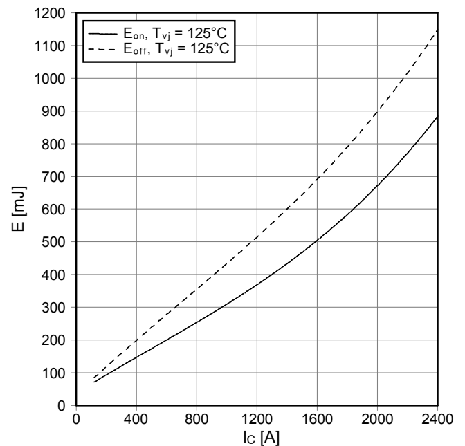
Schaltverluste IGBT-Wechselr. (typisch) switching losses IGBT-inverter (typical) E_{on} = f(I_c), E_{off} = f(I_c) V_{GE} = \pm 15\text{ V}, R_{Gon} = 0.68\ \Omega, R_{Goff} = 0.8\ \Omega, V_{CE} = 900\text{ V}
